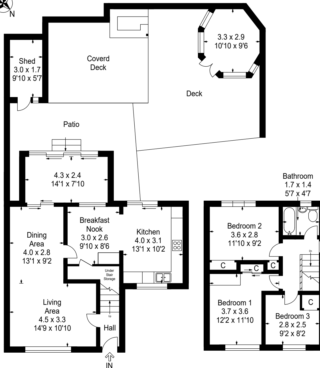
Ground Floor
